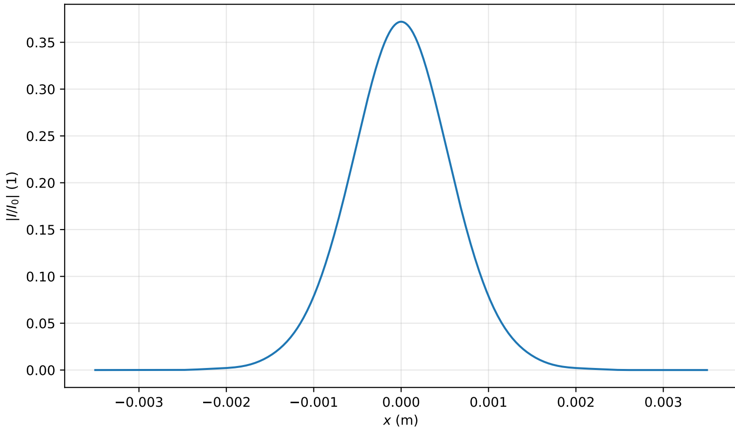
Intensity profile I(x, y = 0, z = 3.662m)/I_0 , P_{in}=0.4P_{cr} , artificial time
